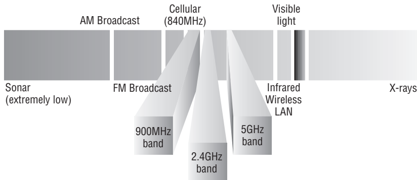
FIGURE 12.1 Unlicensed frequencies
