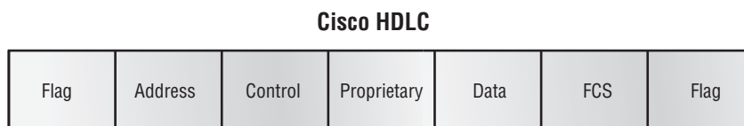
FIGURE 14.7 Cisco HDLC frame format
