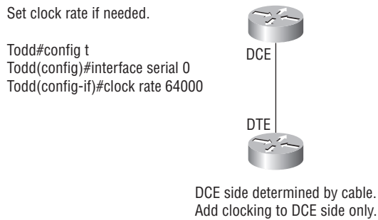
FIGURE 4.5 Providing clocking on a nonproduction network
