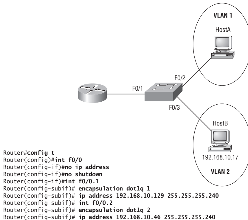
FIGURE 9.12 Inter-VLAN example 4
