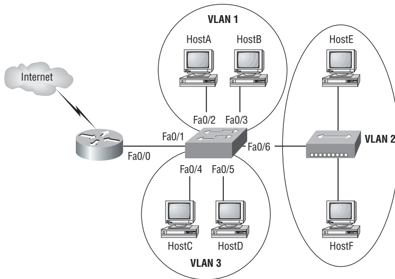
FIGURE 9.10 Inter-VLAN example 2
