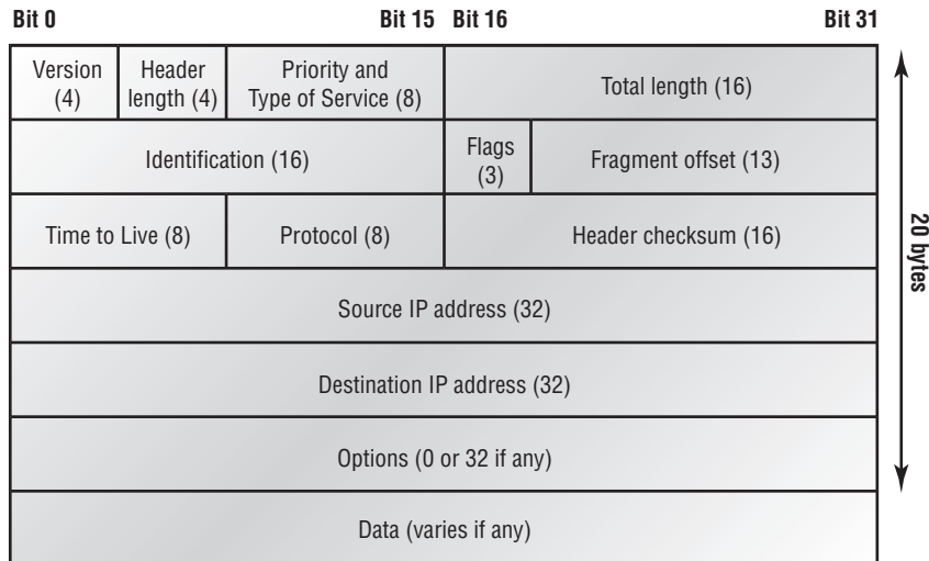
FIGURE 2.6 IP header
