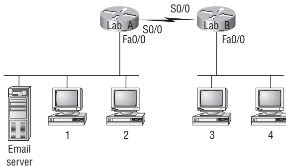
FIGURE 6.8 Testing basic routing knowledge
