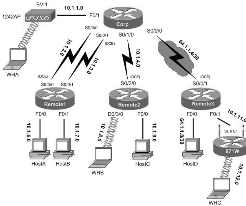
FIGURE 11.6 Our internetwork with new addressing
