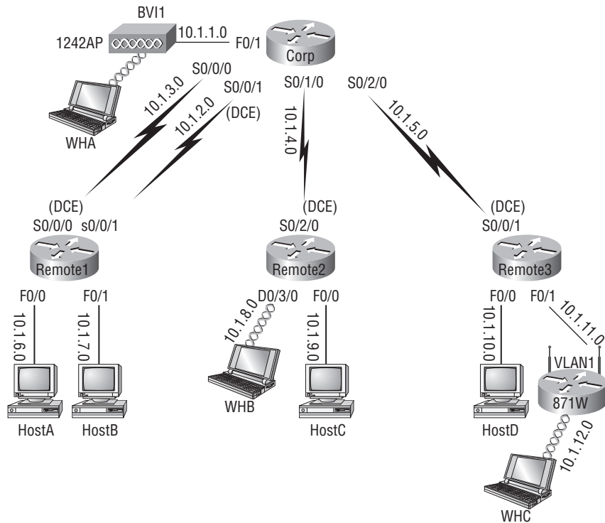
FIGURE 7.3 Our internetwork
