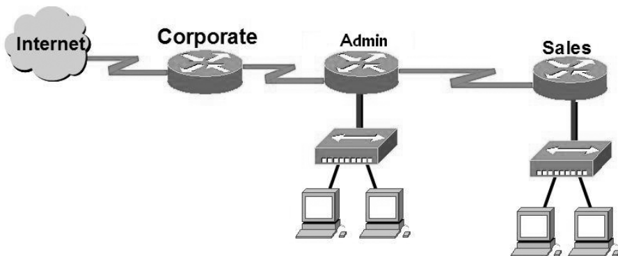
FIGURE 11.4 NAT example
