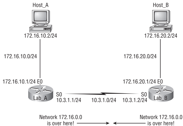
FIGURE 7.2 EIGRP auto-summarization
