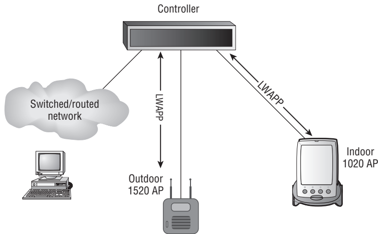
FIGURE 12.7 Split-MAC architecture
