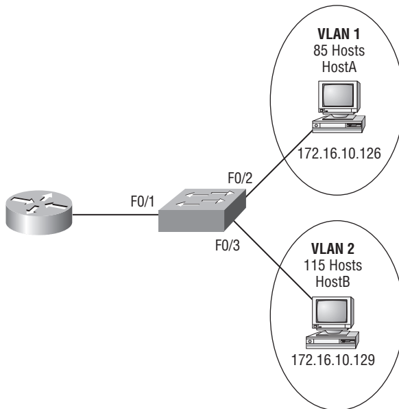
FIGURE 9.11 Inter-VLAN example 3
