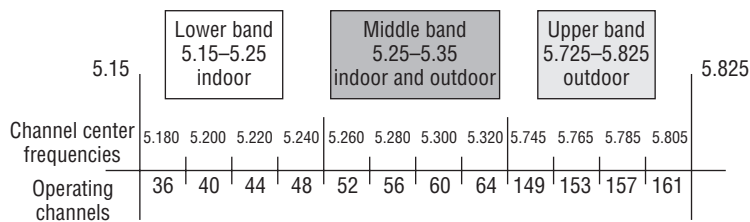
FIGURE 12.4 UNII 5GHz band has 12 non-overlapping channels (U.S.).
