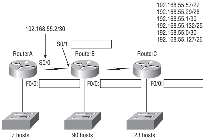
FIGURE 3.11 Solution to VLSM design example 1
